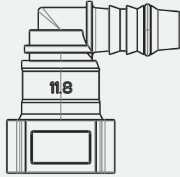
MS4108 ELBOW QUICK CONNECTOR x 1
